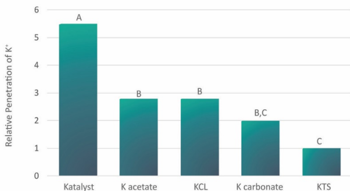
K+ Cuticle Penetration
